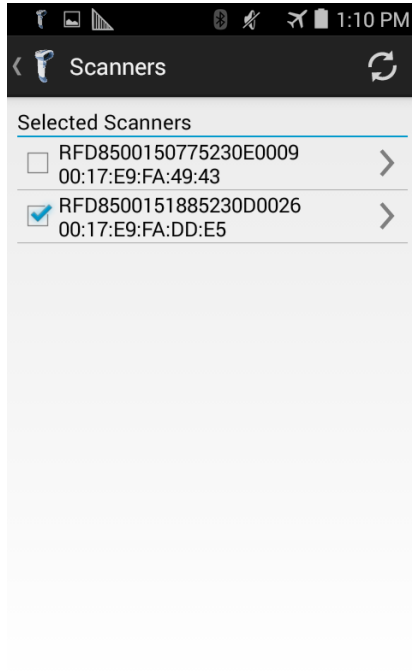
Figure 5-2 Scanners Screen
