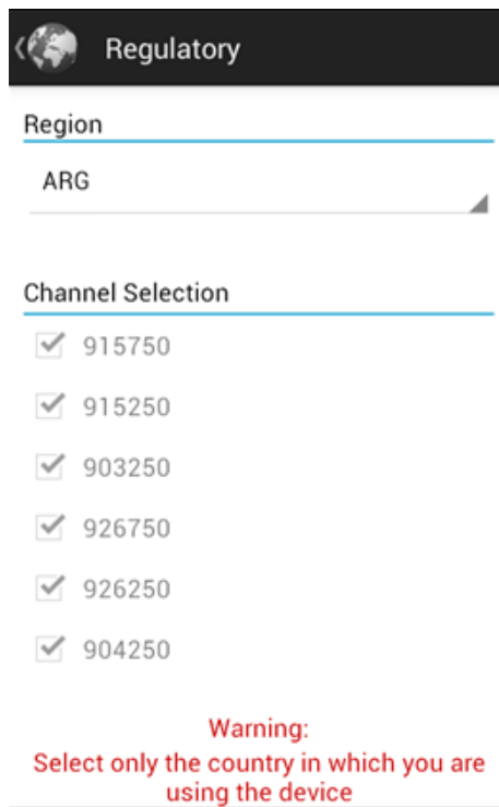
Figure 3-12 Settings - Regulatory
