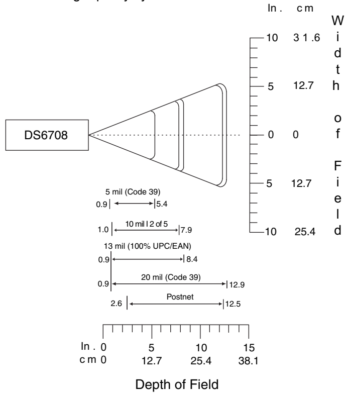
Figure 2-7 DS6708 Digital Scanner Decode Zone for 1D Bar Codes
