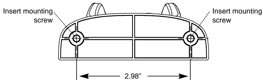
Figure 1-9 Wall Mounting Template
