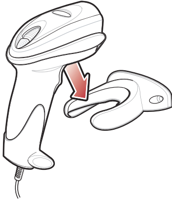
Figure 1-8 Securing the Wall Mount
