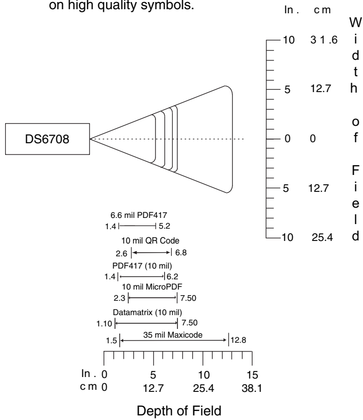
Figure 2-8 DS6708 Digital Scanner Decode Zone for 2D Bar Codes
